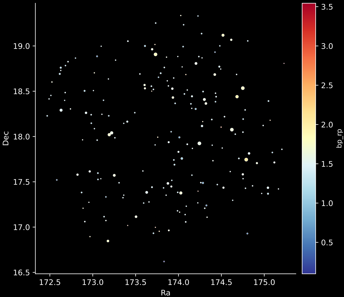
APOGEE DR17 Field: [K2_C13_183-16_btx] Stars: 192
