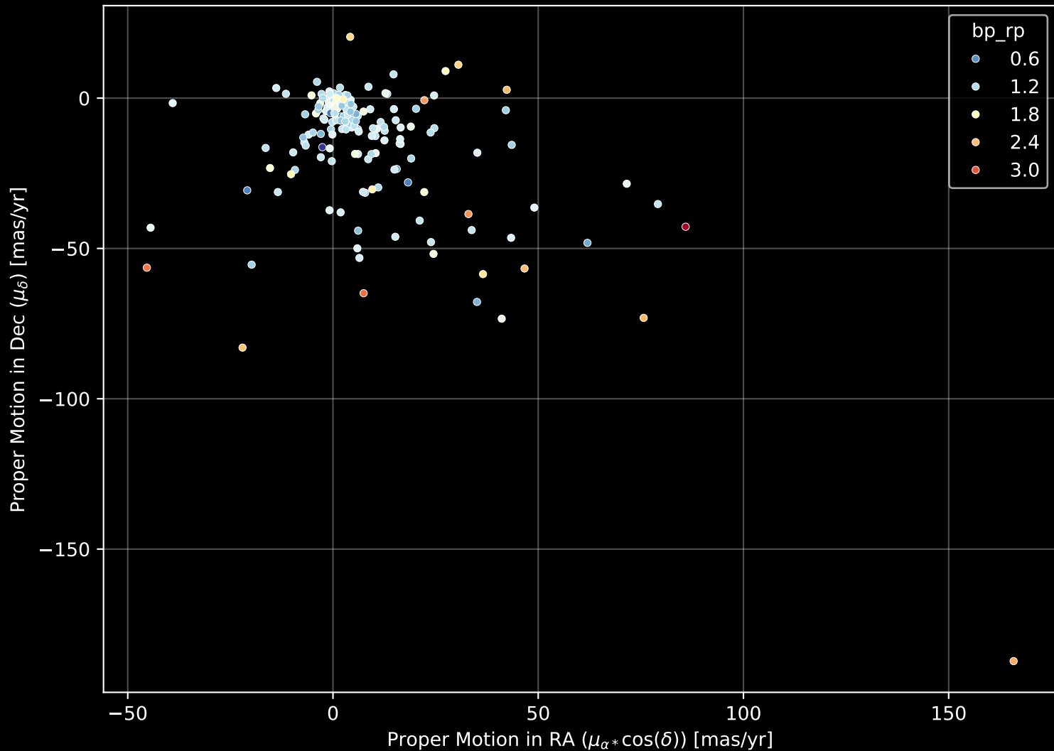
APOGEE DR17 Field: [K2_C13_183-16_btx] Proper Motion Diagram (n= 192)
