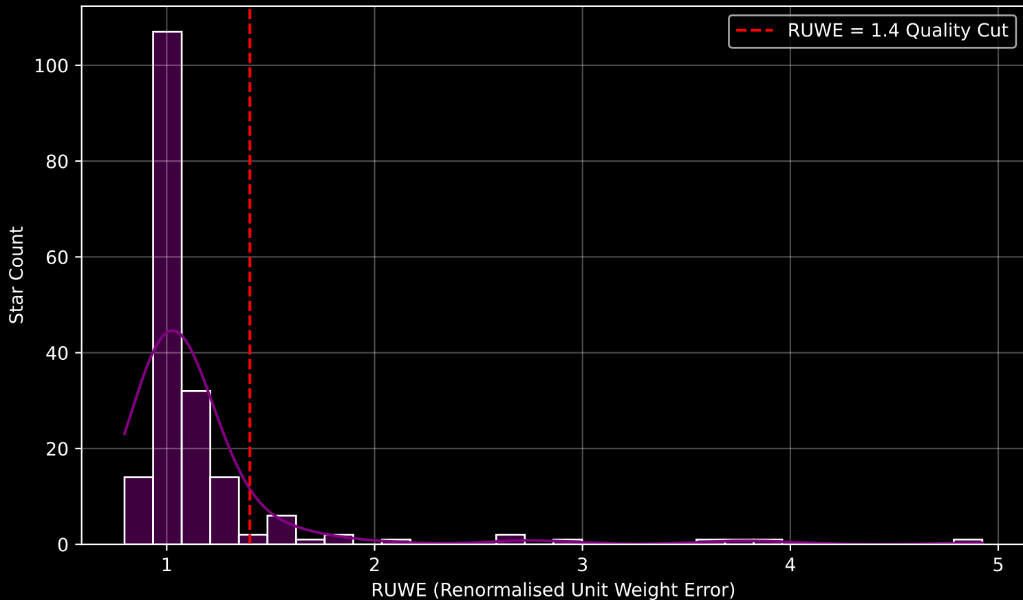
GAPOGEE DR17 Field [K2_C13_183-16_btx] RUWE Distribution (n= 186)
