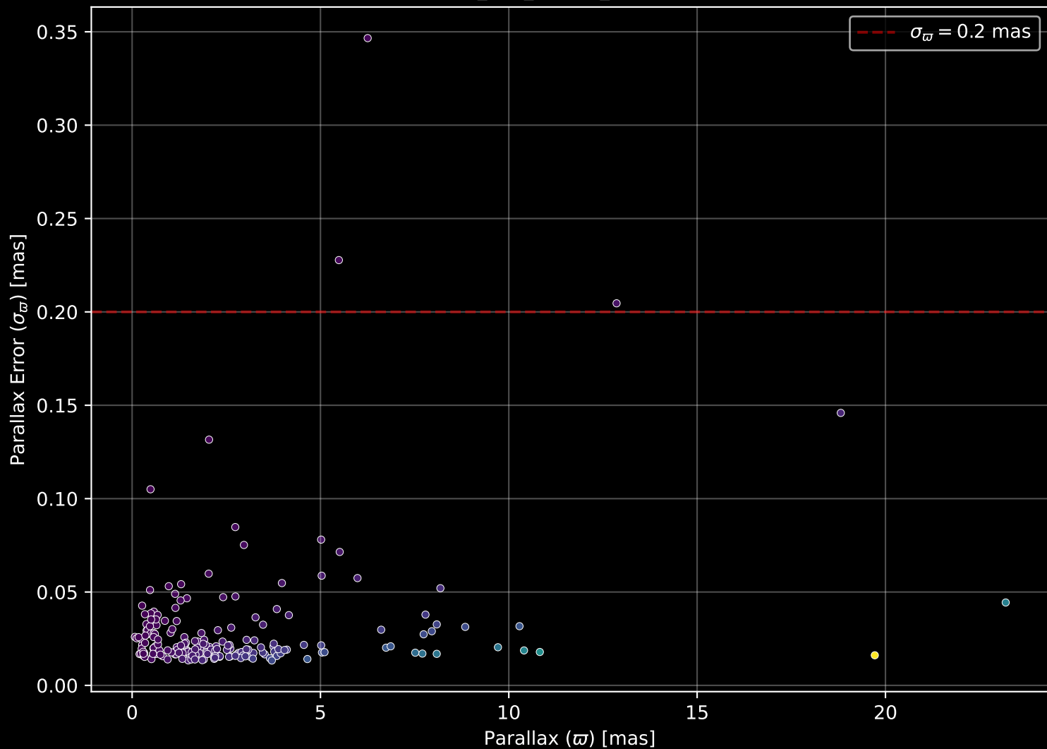
APOGEE DR17 Field: [K2_C13_183-16_btx] Parallax Quality (n= 192)
