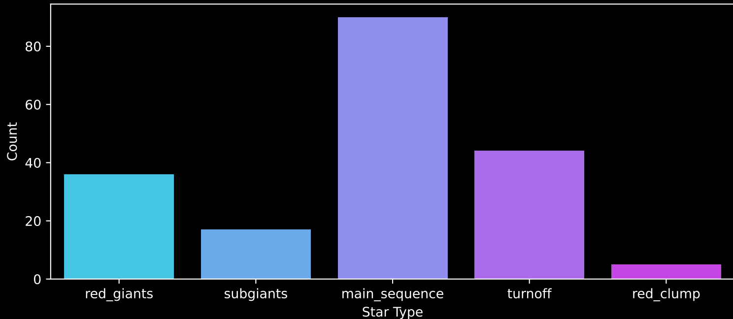
APOGEE DR17 Field: [K2_C13_183-16_btx] Count plot of Star Type
