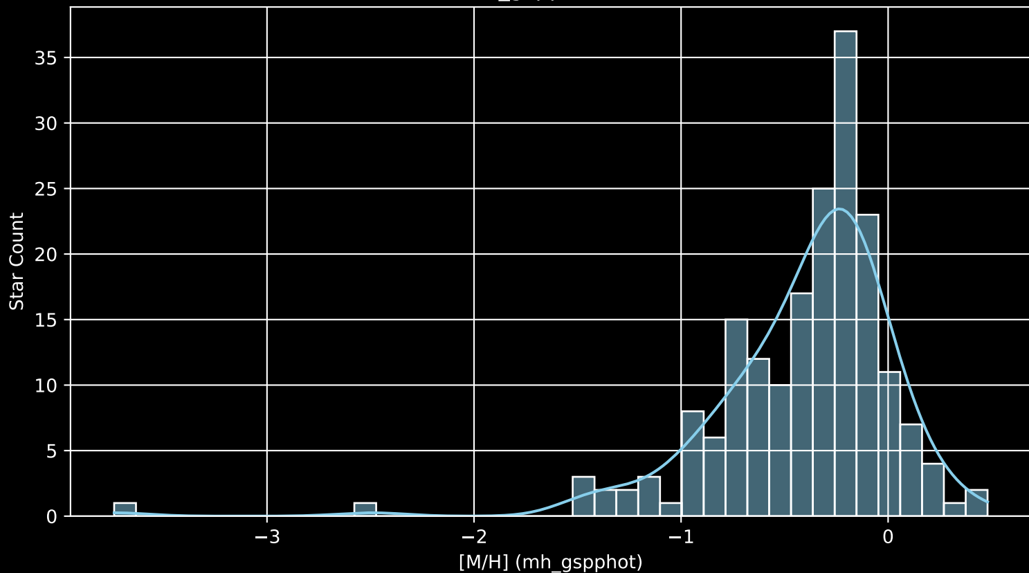
APOGEE DR17 Field: [K2_C13_183-16_btx [M/H] (mh_gspphot) (n= 191)
